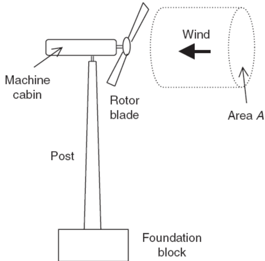
Figure 12-3. Schematic of a wind turbine.
