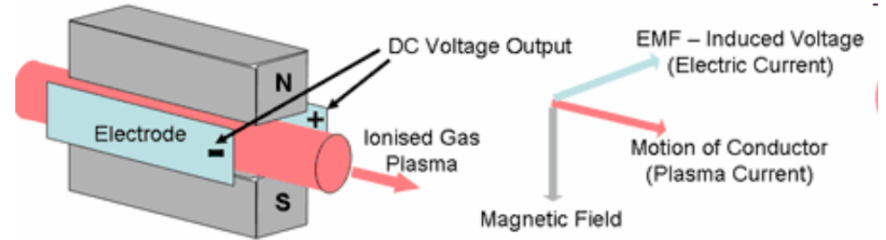
Magneto hydrodynamic Power Generation (Principle)
